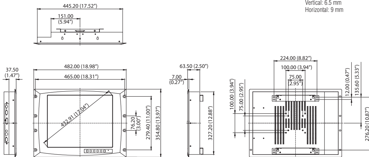
Panel Cut-out Dimensions: 451 x 333 mm (17.75" x 13.11")
